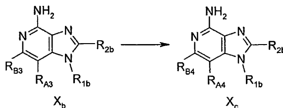
Reaction Scheme VI
